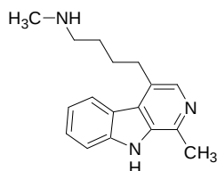
C 17 H 21 N 3 (1)
